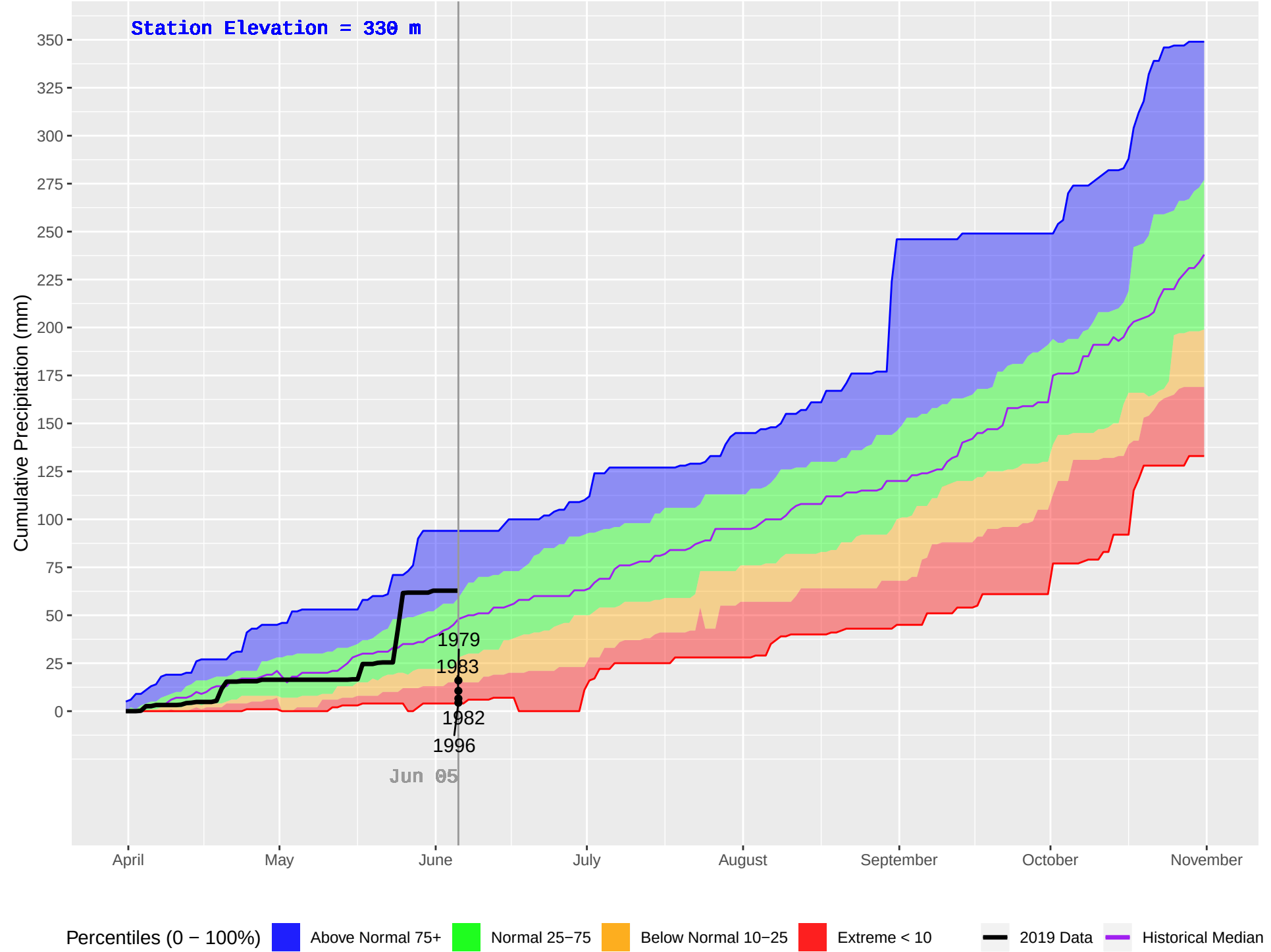
D'ARCY (292) : Historical (1978–2018), Current (2019) Daily Cumulative Precipitation
