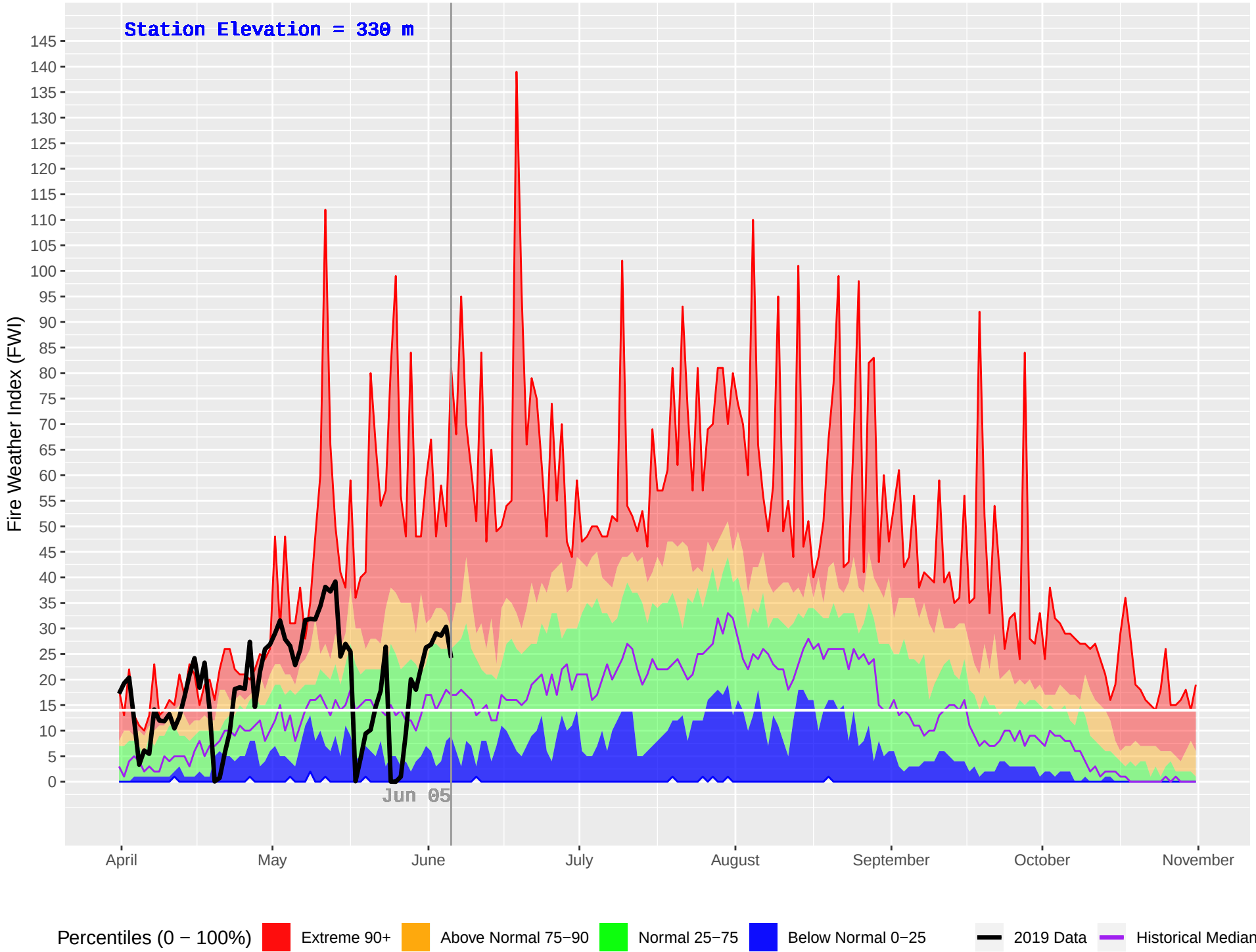
D'ARCY (292) : Historical (1978–2018) and Current (2019) Daily Fire Weather Index (FWI)
