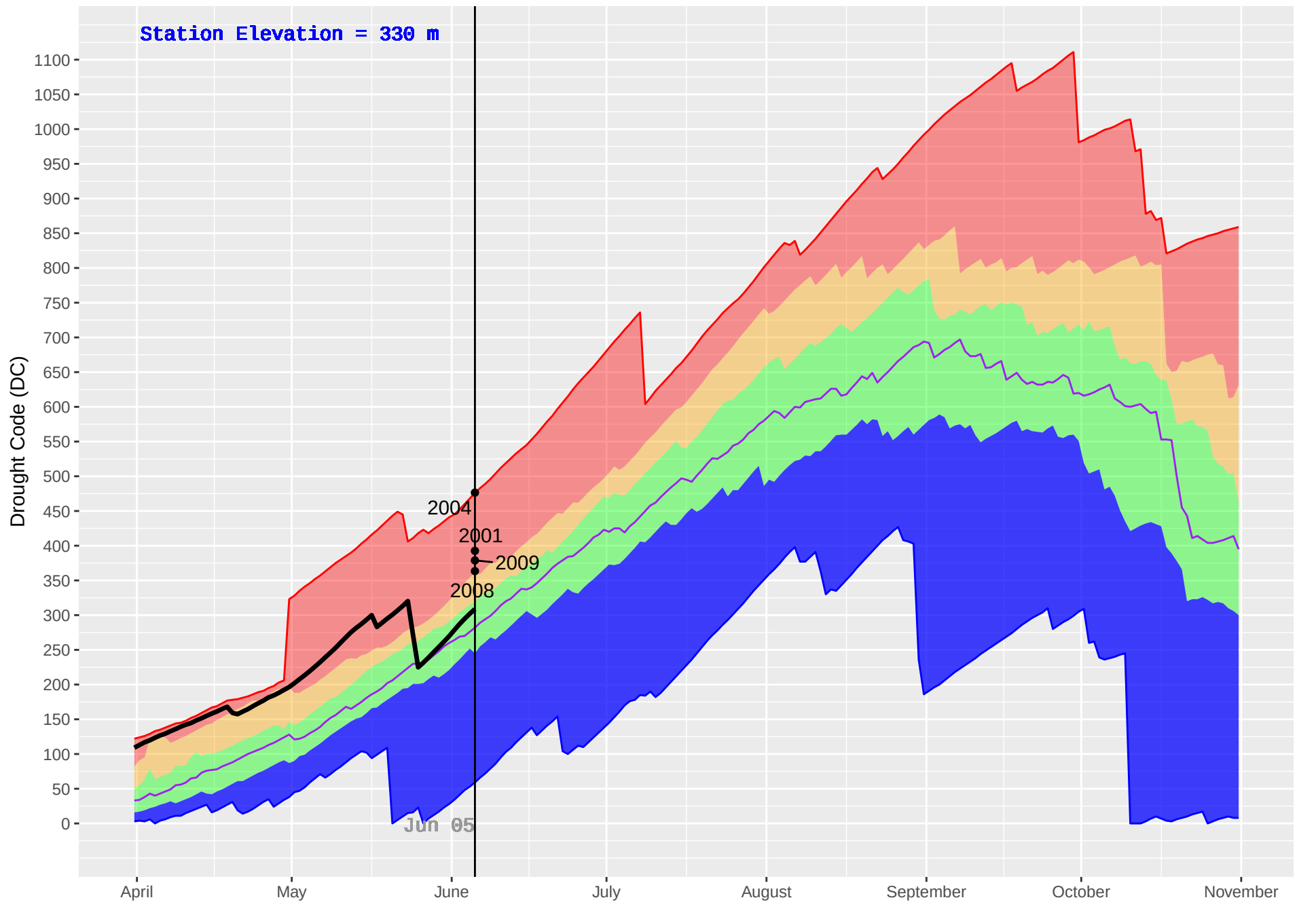
D'ARCY (292) : Historical (1978–2018) and Current (2019) Daily Drought Code (DC)
