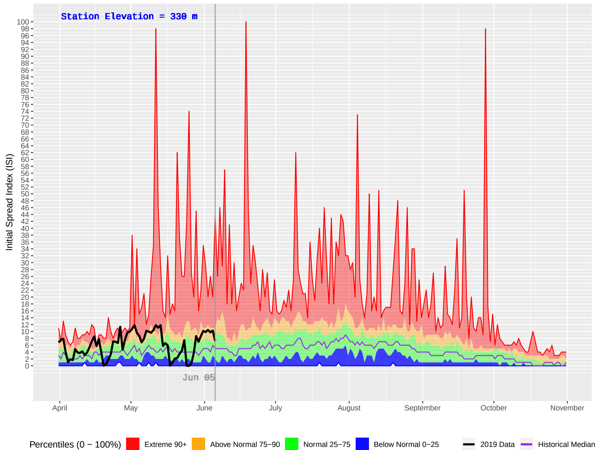
D'ARCY (292) : Historical (1978–2018) and Current (2019) Daily Initial Spread Index (ISI)
