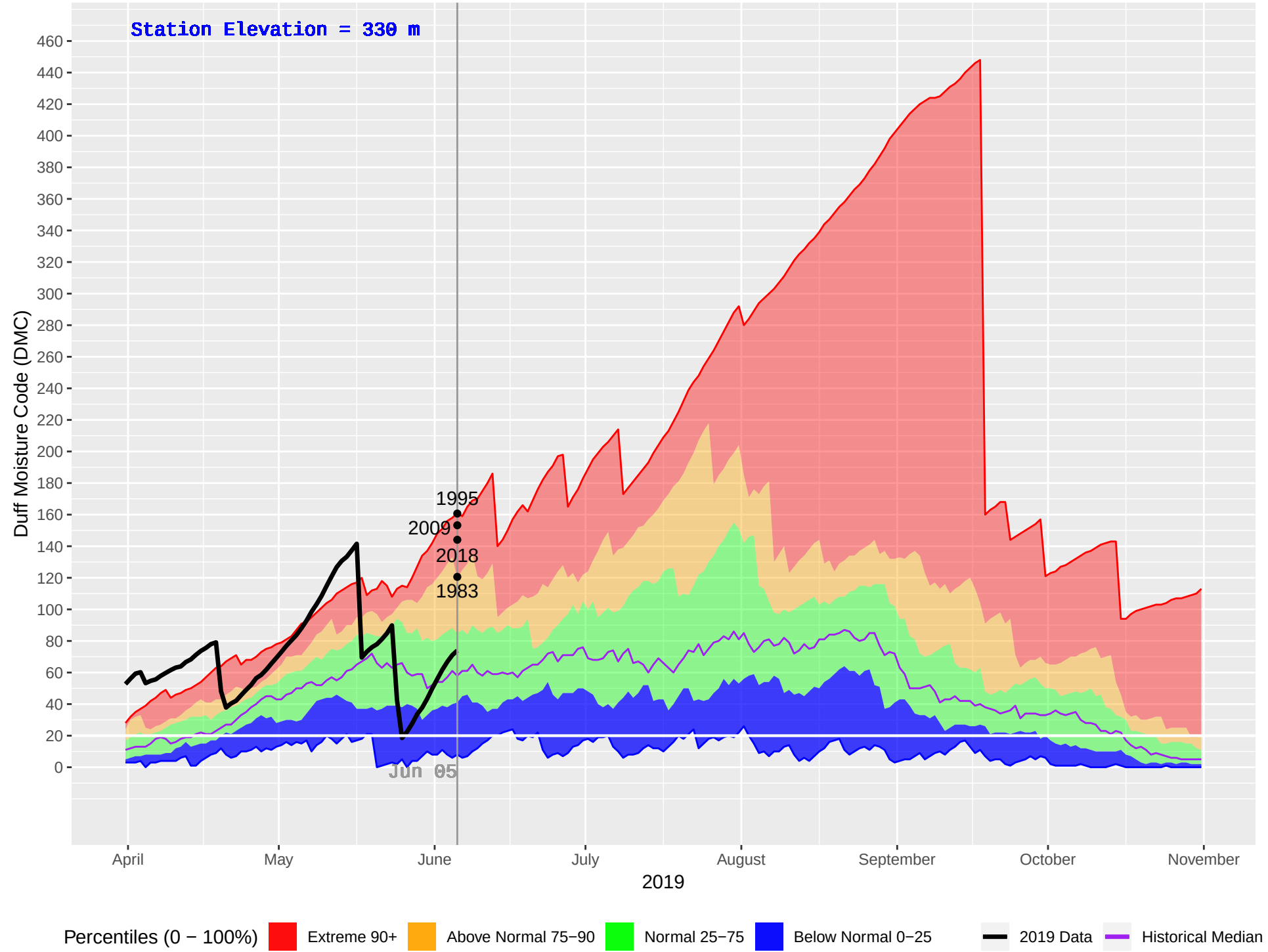
D'ARCY (292) : Historical (1978–2018), Current (2019) Daily Duff Moisture Code (DMC)
