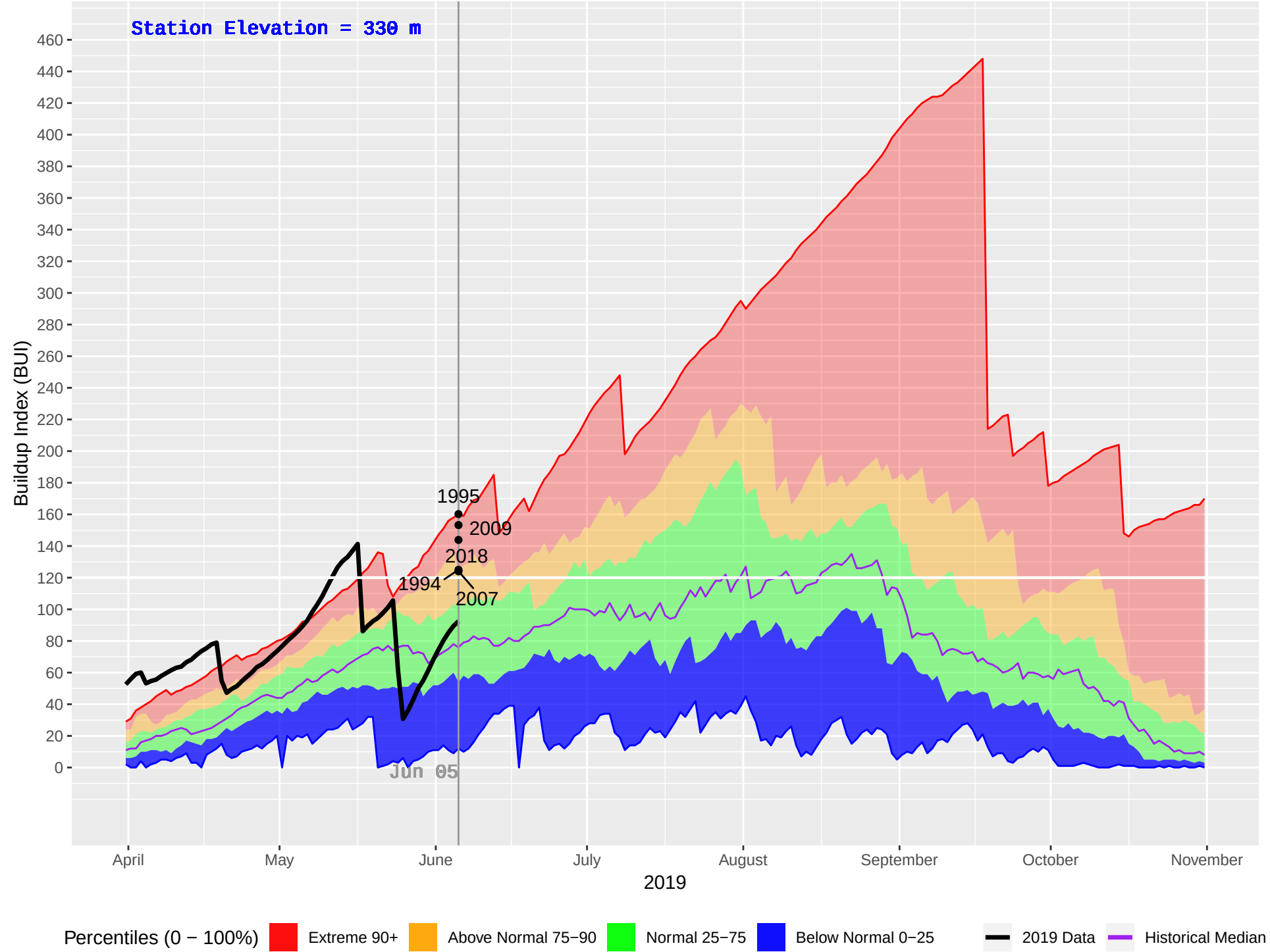
D'ARCY (292) : Historical (1978–2018), Current (2019) Daily Buildup Index (BUI)
