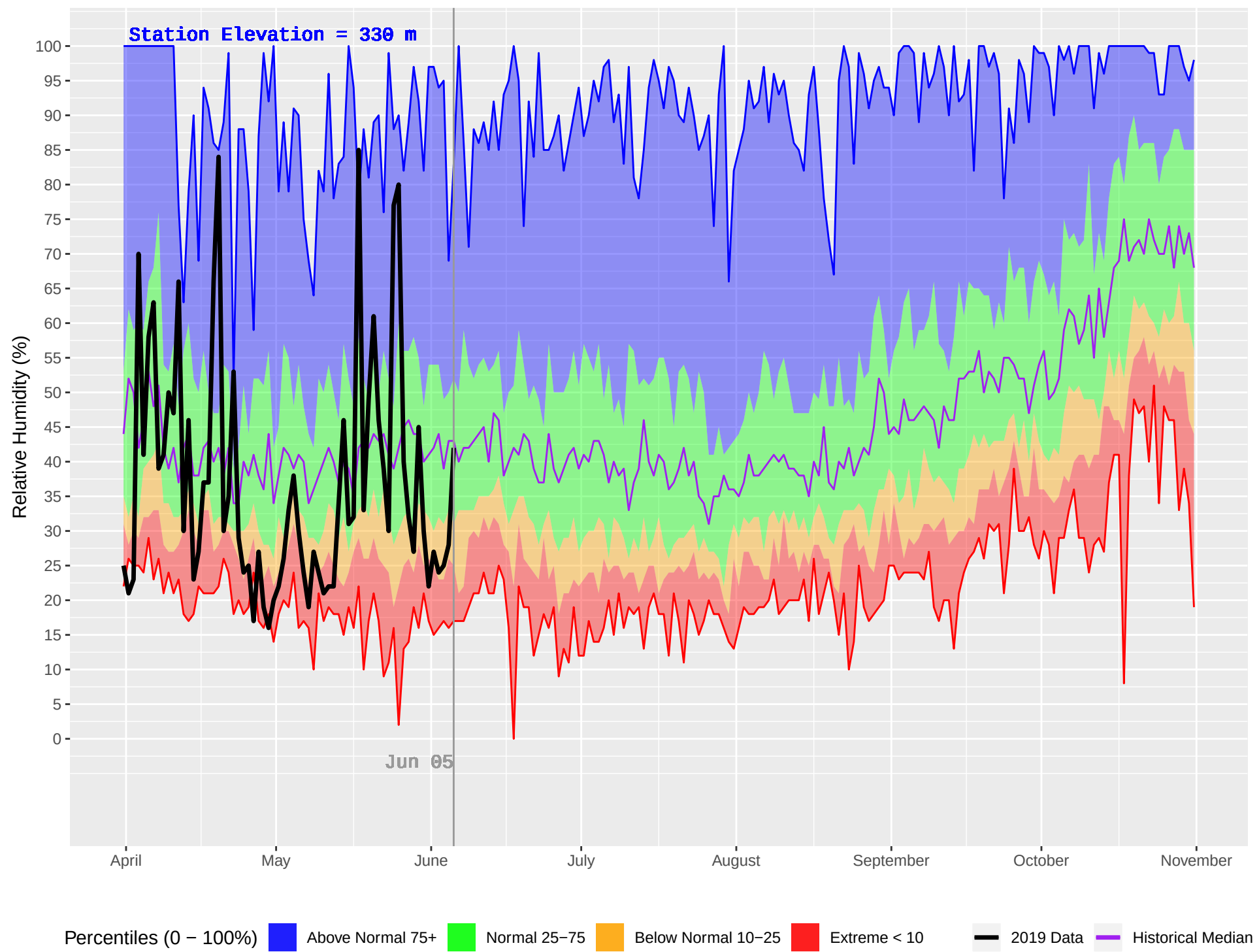
D'ARCY (292) : Historical (1978–2018) and Current (2019) Daily Relative Humidity
