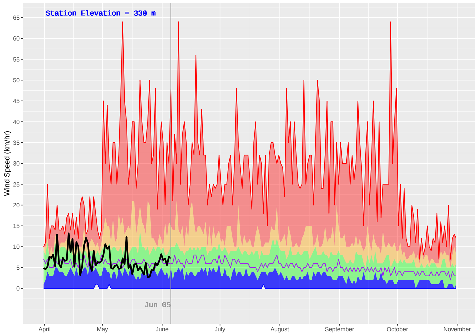
D'ARCY (292) : Historical (1978–2018) and Current (2019) Daily Wind Speed
