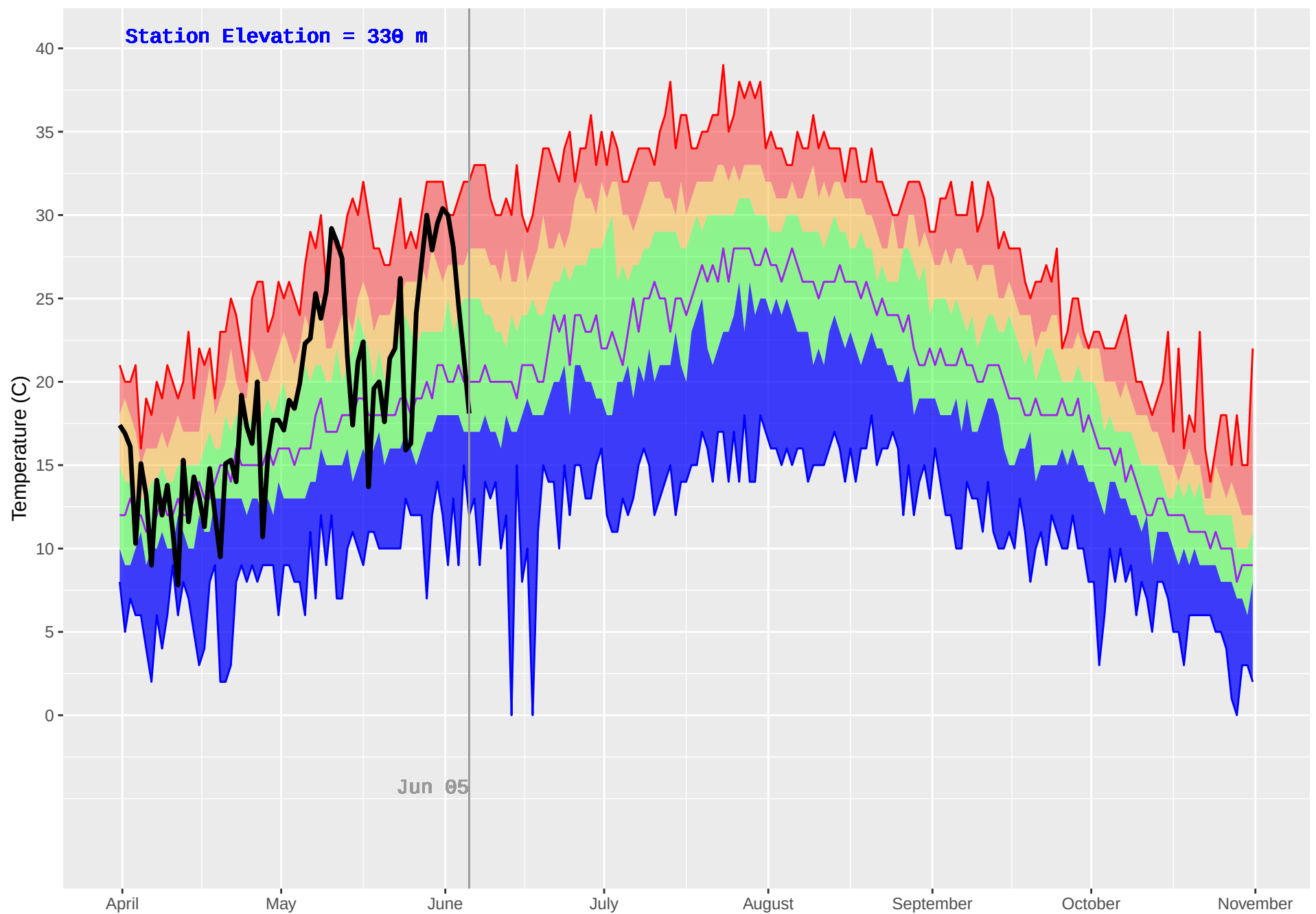
D'ARCY (292) : Historical (1978–2018) and Current (2019) Daily Temperature
